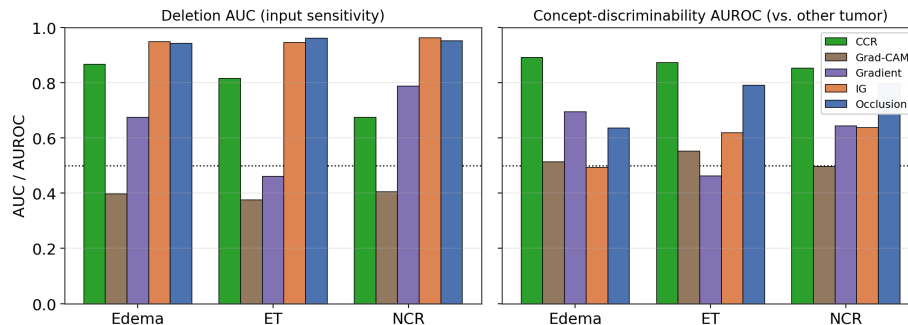
Fig. 5. The ranking inverts across the two axes (per concept, BraTS test). Left: deletion AUC (input sensitivity)—integrated gradients and occlusion dominate. Right: concept-discriminability AUROC (concept vs. other tumor; dotted line = 0.5 chance)—CCR alone rises to the top while the sensitivity methods fall toward chance. A clinical concept explanation needs the right axis.
