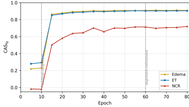
Fig. 8. CAS fg across the three-phase curriculum (dashed lines: phase boundaries). Alignment emerges only after \mathcal{L}_{\text{align}} activates at epoch 11, directly mirroring the A1 ablation.
